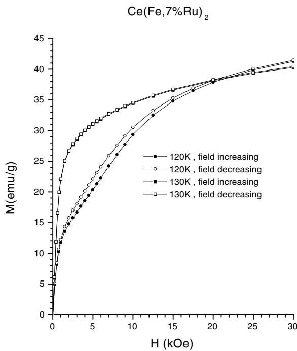
Figure 6. M-H curves for Ce(Fe, 7\% Ru)_2 at temperatures of 120 K and 130 K. See the text for details.
