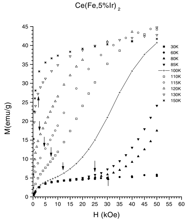
Figure 2. Magnetization versus field plots for \text{Ce}(\text{Fe}, 5\% \text{Ir})_2 at various temperatures. The arrows mark the onset field H_M of the metamagnetic transition. The line for the M-H curve at T = 100 \text{ K} serves as a guide to the eye.
