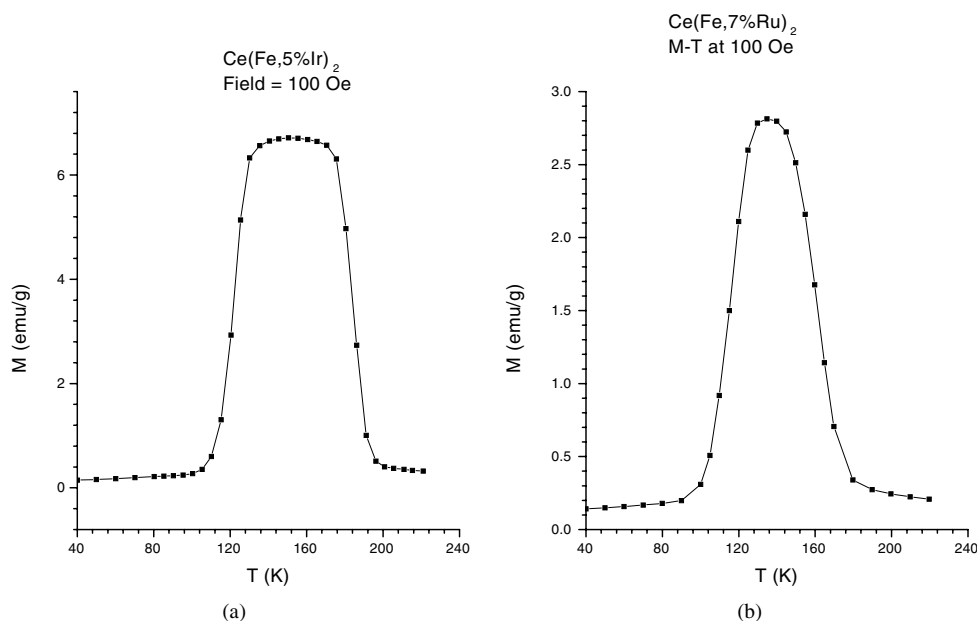
Figure 1. Magnetization versus temperature plots for (a) \text{Ce}(\text{Fe}, 5\% \text{Ir})_2 and (b) \text{Ce}(\text{Fe}, 7\% \text{Ru})_2 .
