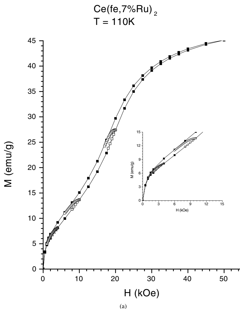
Figure 8. Minor hysteresis loops generated during: (a) the ascending-field cycle for \text{Ce}(\text{Fe}, 7\% \text{Ru})_2 at H = 4 kOe (open triangles), H = 10 kOe (open circles) and H = 20 kOe (open squares); (b) the descending-field cycle for \text{Ce}(\text{Fe}, 7\% \text{Ru})_2 at H = 8 kOe (open squares) and H = 22 kOe (open circles). The envelope curve is represented by solid squares. The measurements were done at T = 110 K. The inset shows an expanded view.
