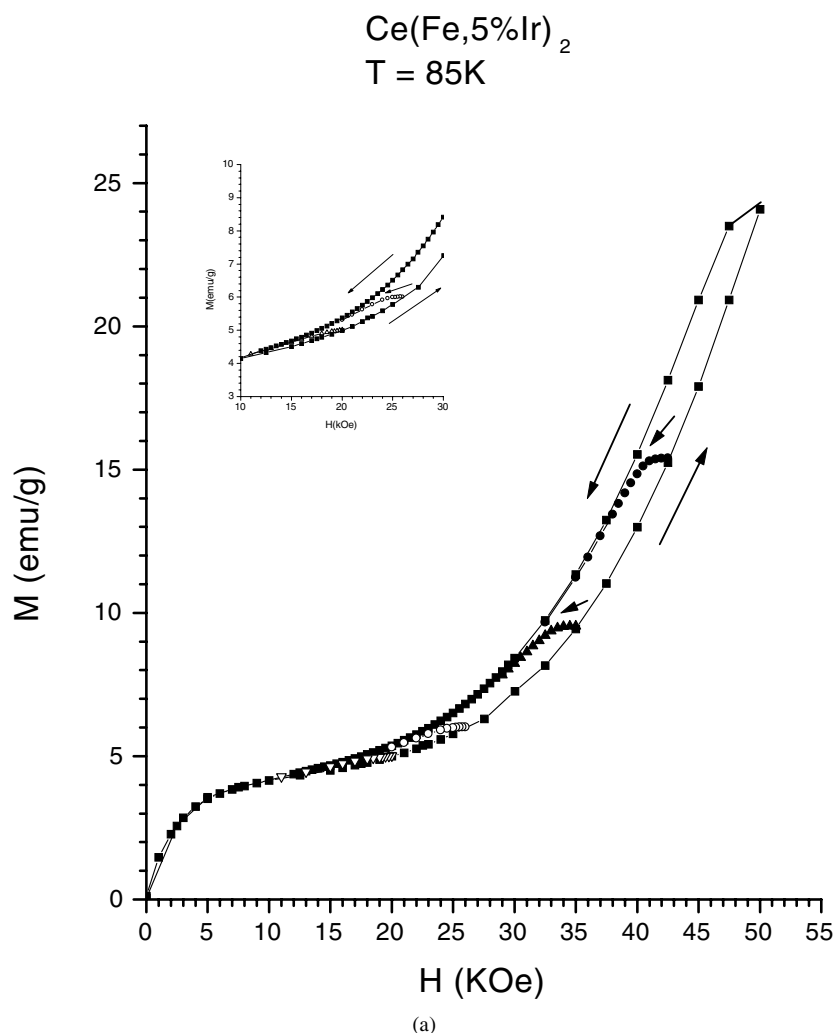
Figure 7. Minor hysteresis loops generated during: (a) the ascending-field cycle for \text{Ce}(\text{Fe}, 5\% \text{Ir})_2 at H = 20 kOe (open triangles), H = 26 kOe (open circles), H = 35 kOe (solid triangles) and H = 42.5 kOe (solid circles); (b) the descending-field cycle for \text{Ce}(\text{Fe}, 5\% \text{Ir})_2 at H = 40 kOe (open squares) and H = 45 kOe (solid triangles). The envelope curve is represented by solid squares. The measurements were done at T = 85 K. The inset shows an expanded view.
