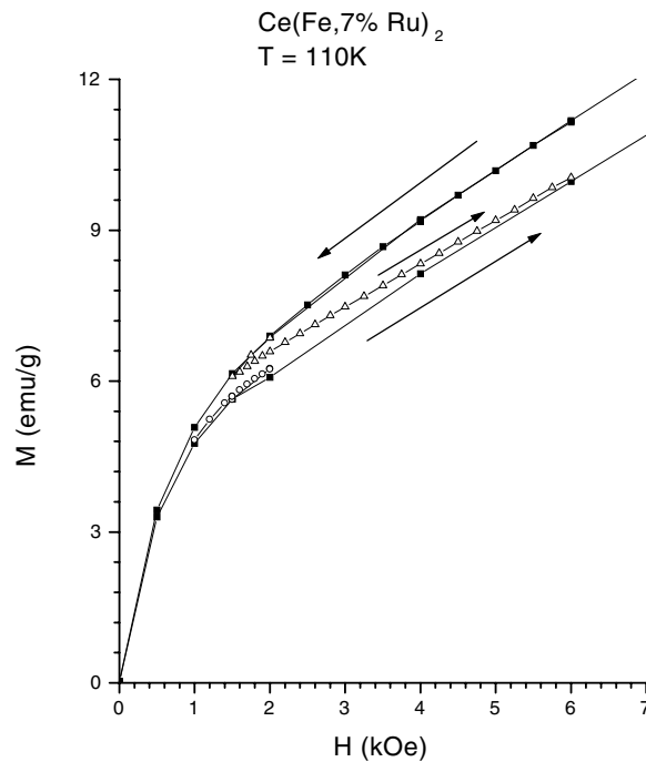
Figure 9. Comparison of minor hysteresis loops generated during the ascending-field cycle ( H = 2\text{ kOe} —open circles) and descending-field cycle ( H = 1.6\text{ kOe} —open triangles) at approximately the same values of the magnetization for \text{Ce}(\text{Fe}, 7\% \text{Ru})_2 at T = 110\text{ K} . The envelope curve is represented by solid squares. See the text for details.
