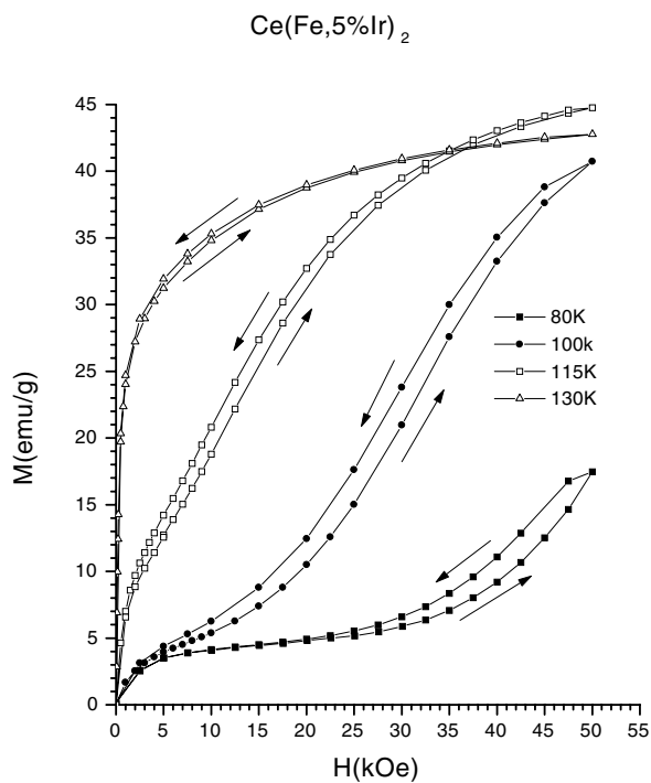
Figure 4. M-H curves for \text{Ce}(\text{Fe}, 5\% \text{Ir})_2 showing hysteresis associated with the metamagnetic transition. The arrows show the direction of field change.
