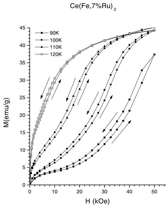
Figure 5. M-H curves for Ce(Fe, 7\% Ru)_2 showing hysteresis associated with the metamagnetic transition. The arrows show the direction of field change.
