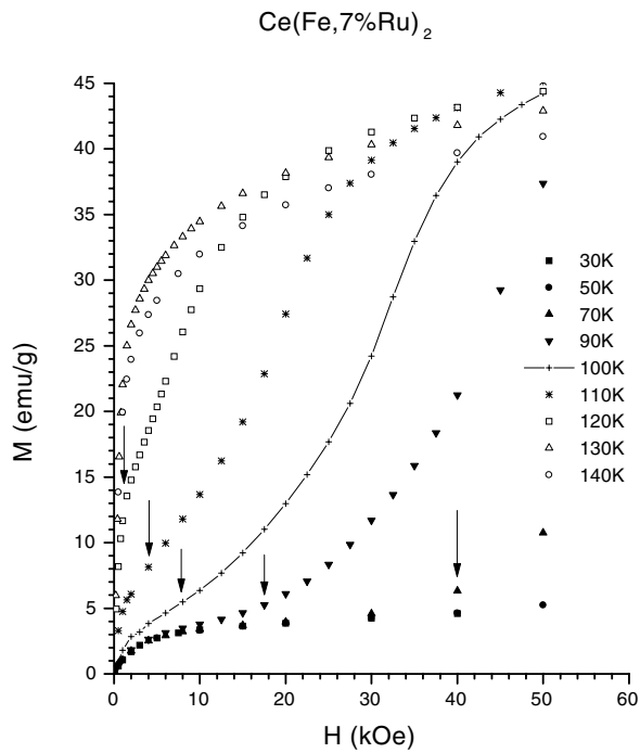
Figure 3. Magnetization versus field plots for \text{Ce}(\text{Fe}, 7\% \text{Ru})_2 at various temperatures. The onset field H_M of the metamagnetic transition is marked by arrows. The line for the M-H curve at T = 100 \text{ K} serves as a guide to the eye.
